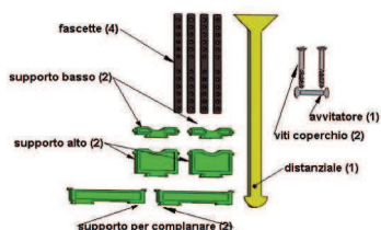
Supporti per complanari Complanar manifold supports
